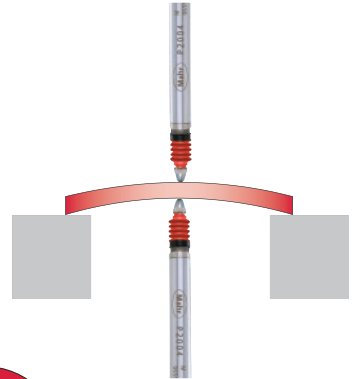
Thickness measurement
